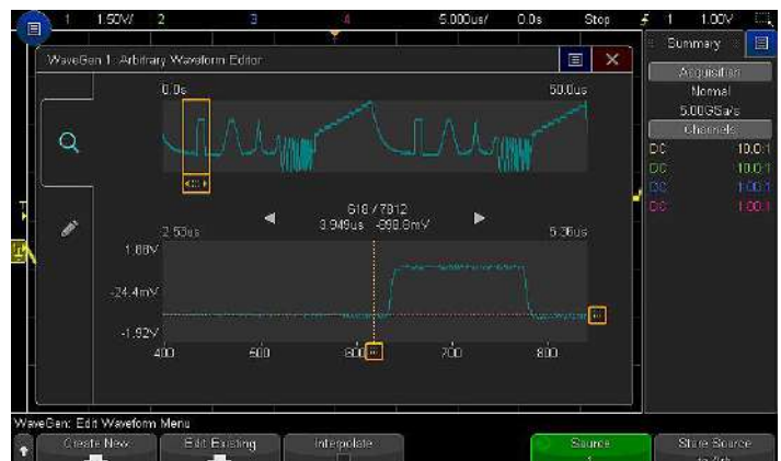
Figure 26. Optional arbitrary waveform generator provides easy access to stimulus. The integrated arbitrary waveform generator makes capturing, modifying and replaying signals simple.
