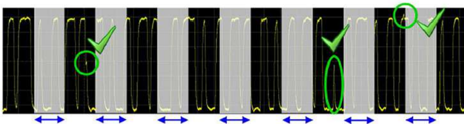
Figure 10. InfiniiVision 3000T X-Series with 1,000,000 waveforms/second. A short dead time increases the probability of capturing infrequent events.
