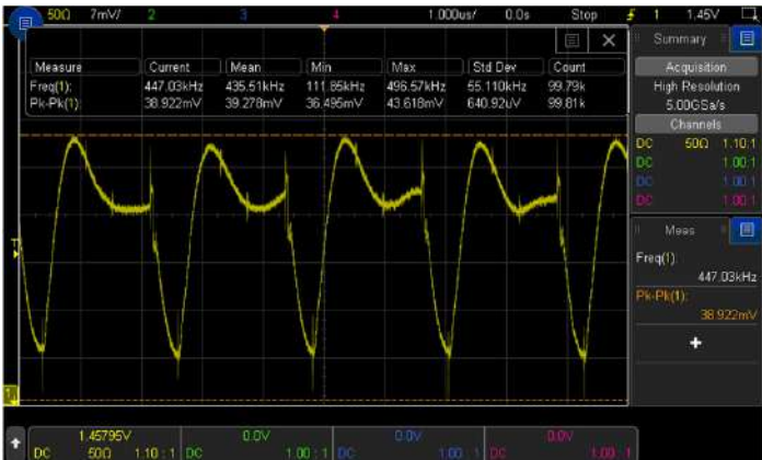
Figure 31a. 3000T X-Series and N7020A acquire not only the power rail ripples but the high frequency transients as well.
